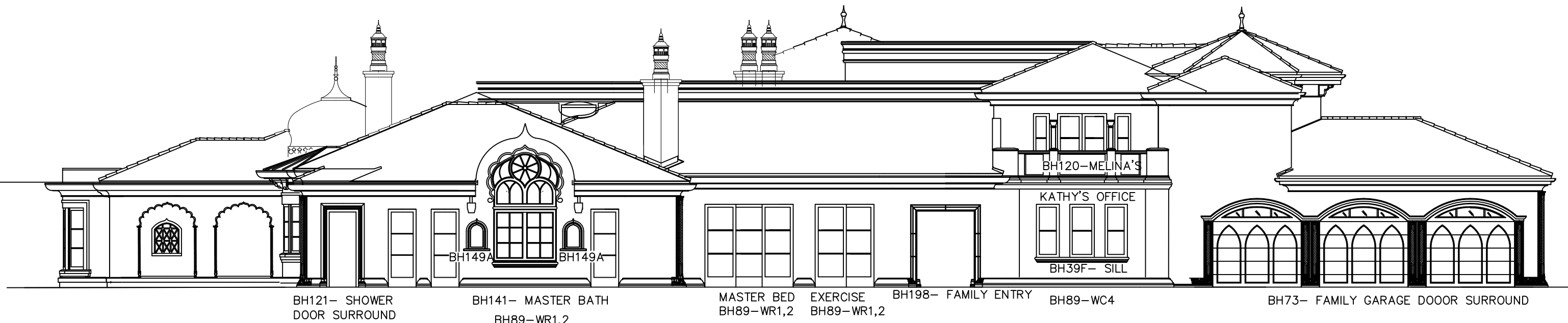
EAST ELEVATION
