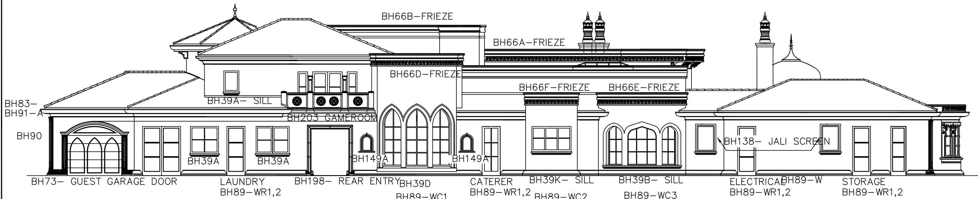
WEST ELEVATION
