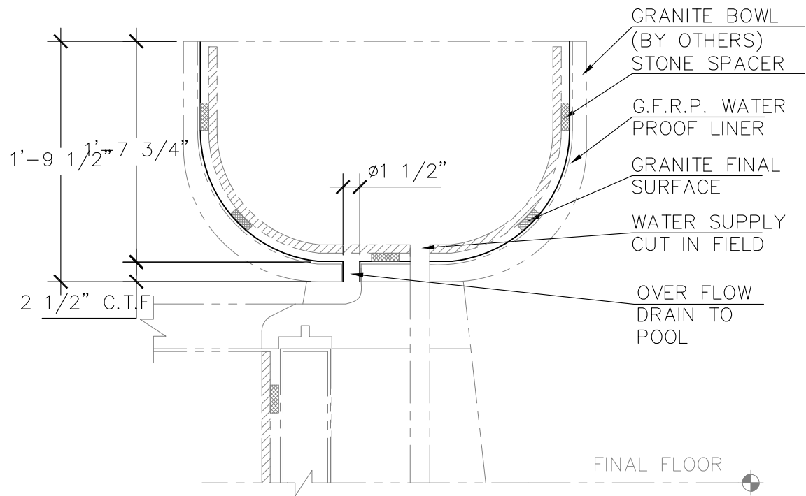
BAPTISM BOWL SECTION - A
