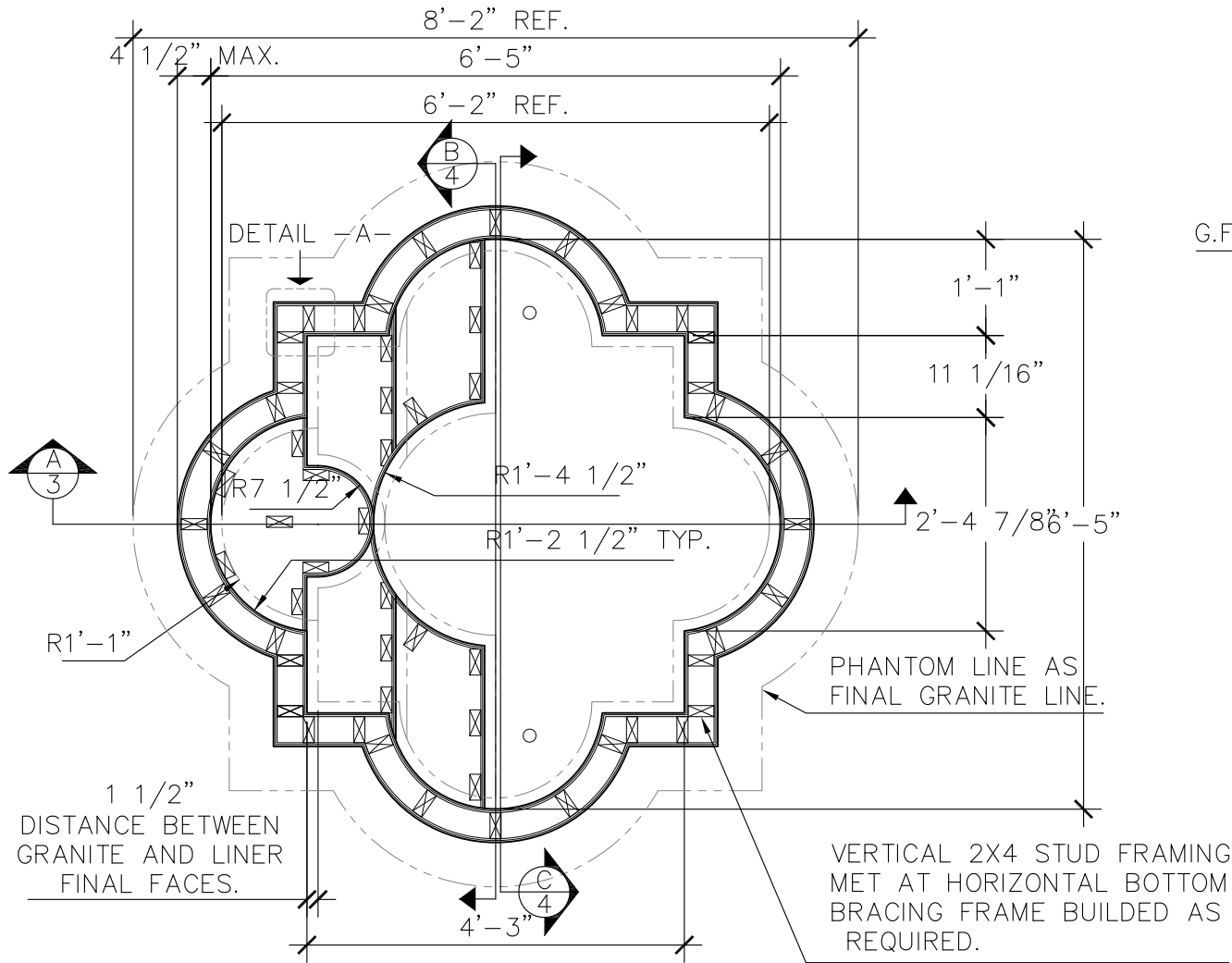
LINER PLAN VIEW
