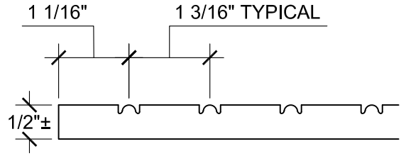
SECTION A
