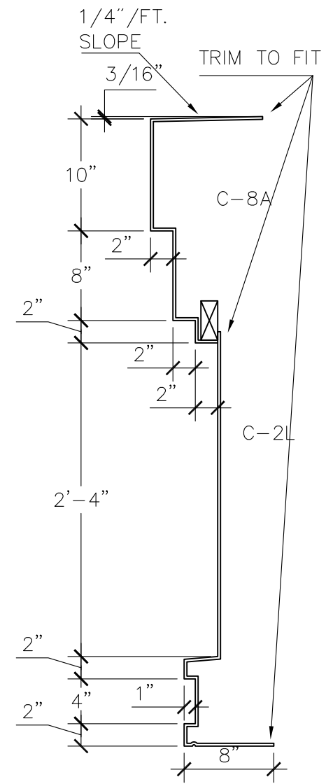
SECTION A SCALE 1" = 1'
