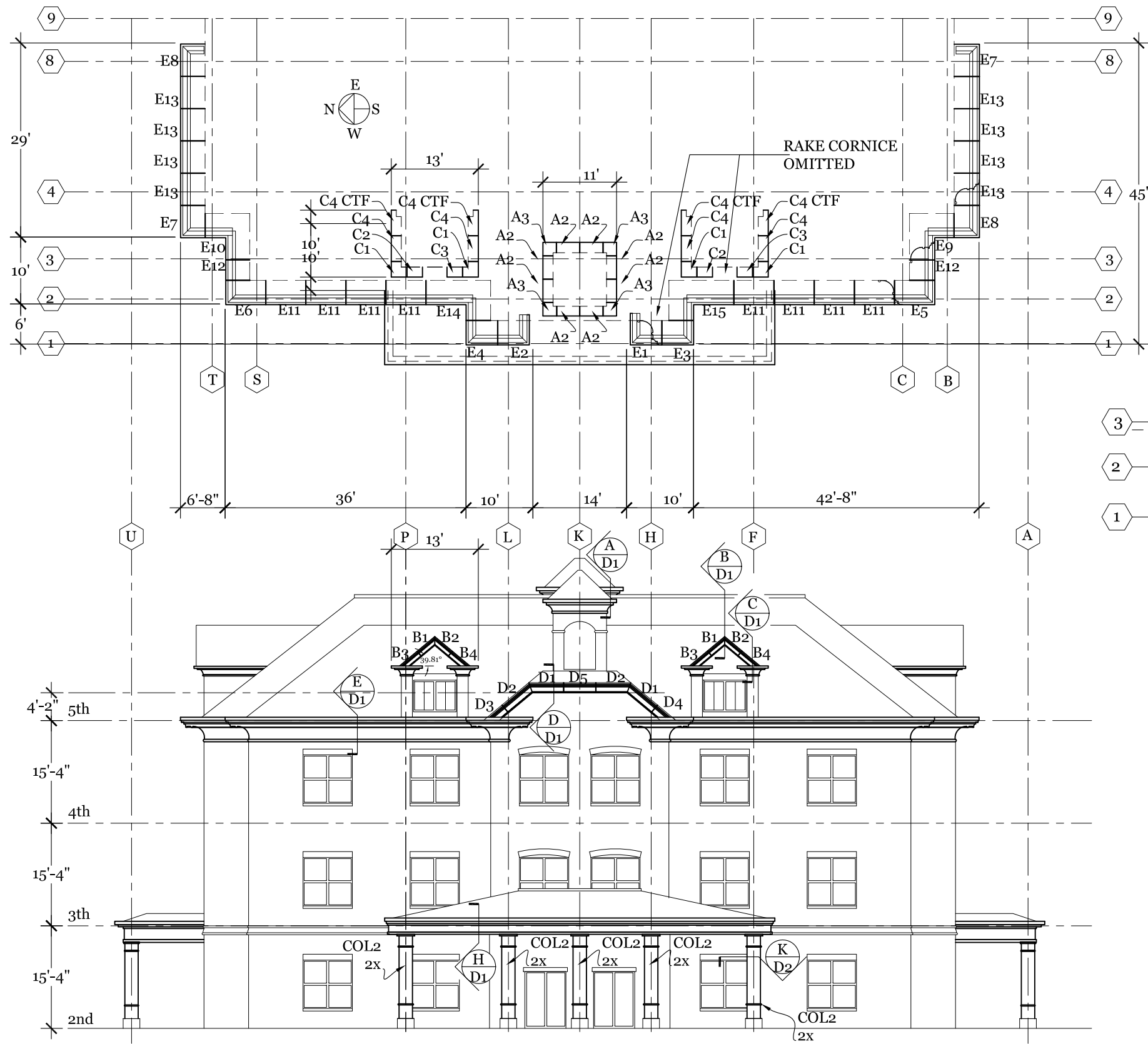
SP3 WEST ELEVATION SETTING PLAN
